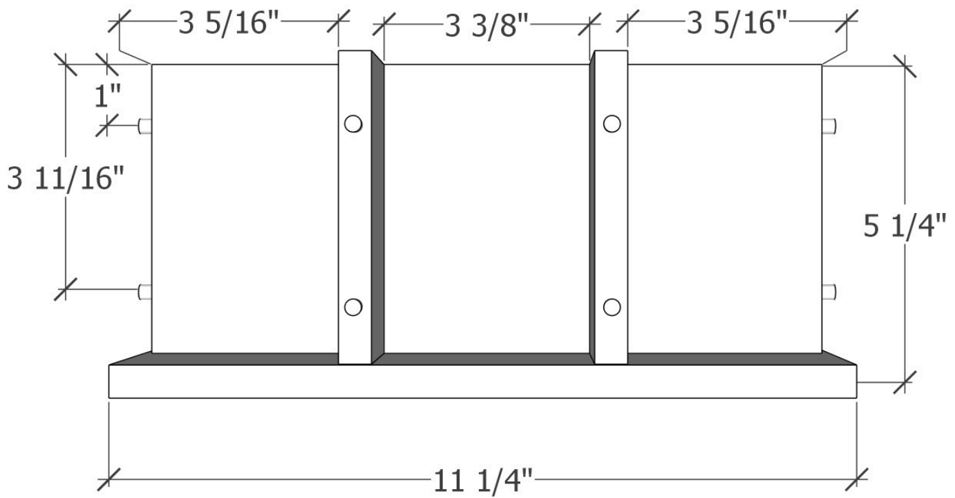
TOP VIEW OF DIVIDERS
