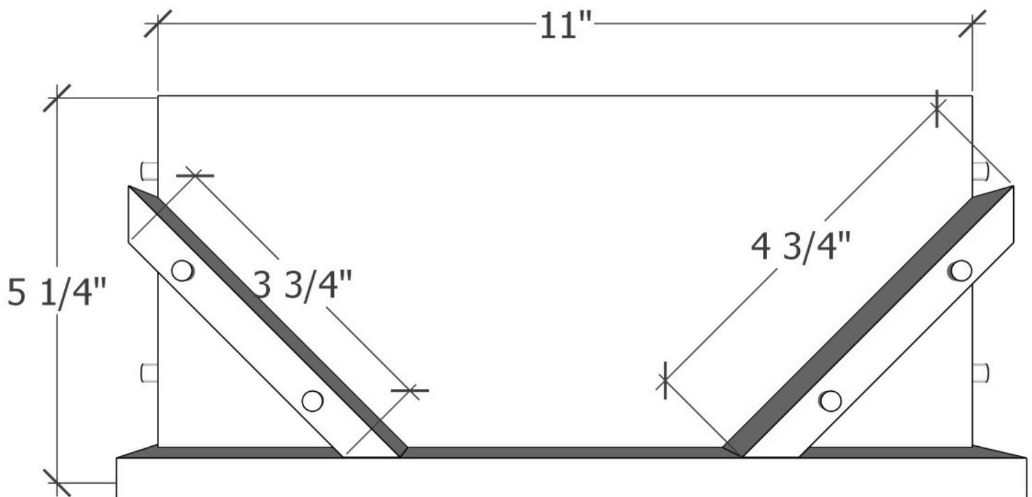
SIDE VIEW OF PLATE DIVIDER WITH PLATE SUPPORTS
