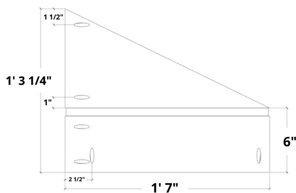
DIVIDER SHELF PANEL (QTY 1)
