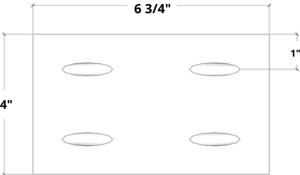
BOX FRONT & BACK - QTY 2
