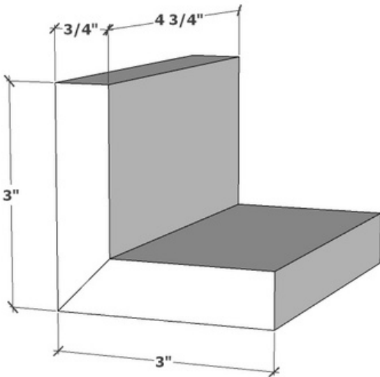
SMALL CORNER SUPPORT - QTY 2
