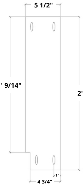
INSIDE VERTICAL PIECES - QTY 2
