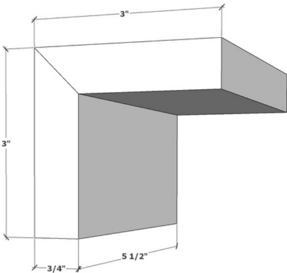
LARGE CORNER SUPPORT - QTY 2
