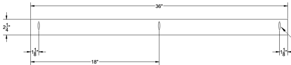
BACK BOARD - LARGE CLAMP HOLDER
