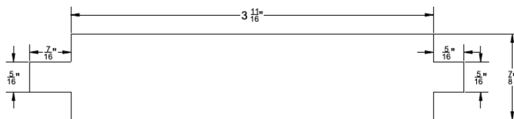
CORNER CLAMP HOLE DETAIL (NTS)
