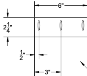
FRONT BOARD SMALL CLAMP HOLDER — Pocket Holes (TYP)
