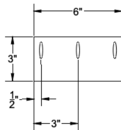
TOP BOARD SMALL CLAMP HOLDER
