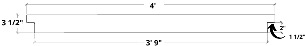
BASE SLATS (NOTCHED) - QTY 2
