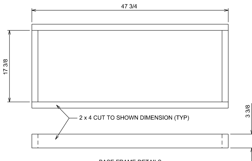
BASE FRAME DETAILS
