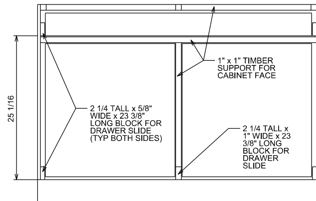
CABINET BACK VIEW - FRAMING
