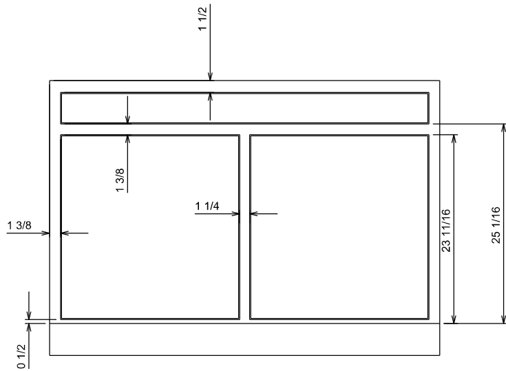
FACE TRIM DETAILS
