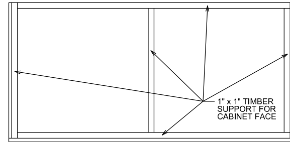
CABINET TOP VIEW - FRAMING
