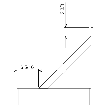
DRAWER SIDE DETAIL
