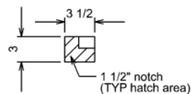
LEG TOP VIEW
