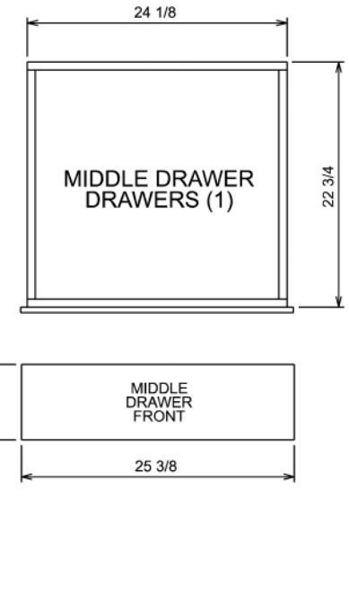
DRAWER DETAILS
