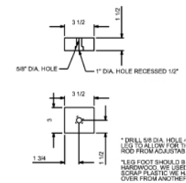
DETAIL A ADJUSTABLE LEG
