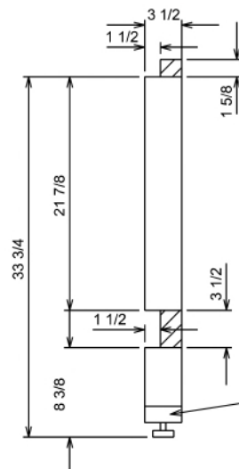
LEG SIDE VIEW B
