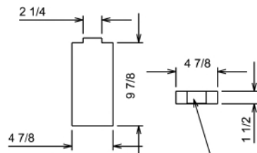
DETAIL B KREG K5 JIG INSERT
