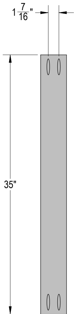
⑤ HEADBOARD / FOOTBOARD CENTER RAIL MATERIAL: PINE/POPLAR QTY: 2
