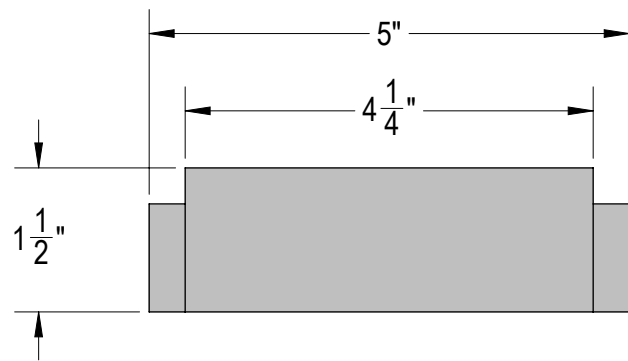
⑫ DRAWER FRONT STILE MATERIAL: POPLAR QTY: 12
