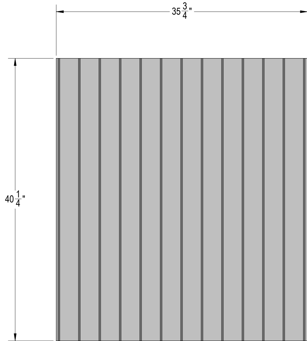
⑦ ⑧ HEADBOARD PANEL MATERIAL: BEADBOARD & 1/4" PLY QTY: 1
