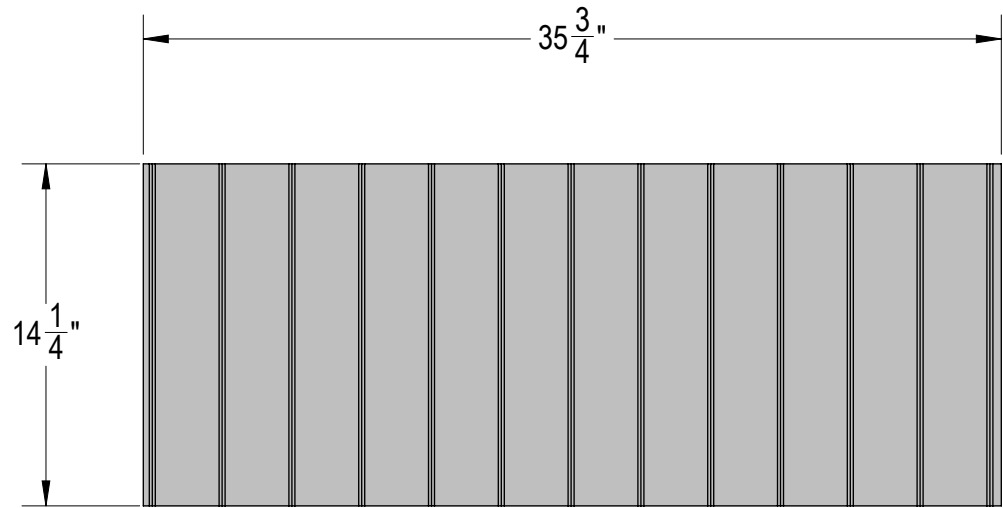
⑨ ⑩ FOOTBOARD PANEL MATERIAL: BEADBOARD & 1/4" PLY QTY: 1
