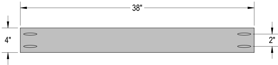
②① DRAWER SLIDE BRACE MATERIAL: 3/4" PLY QTY: 6
