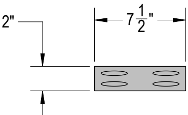
⑫ BED FRAME STILE MATERIAL: POPLAR QTY: 8
