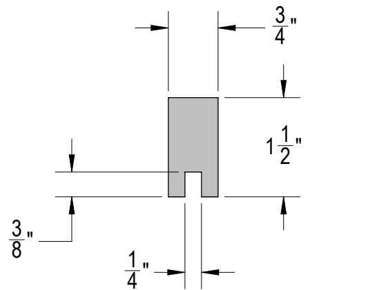
PROFILE DETAIL: DRAWER FRONT RAILS & STILES
