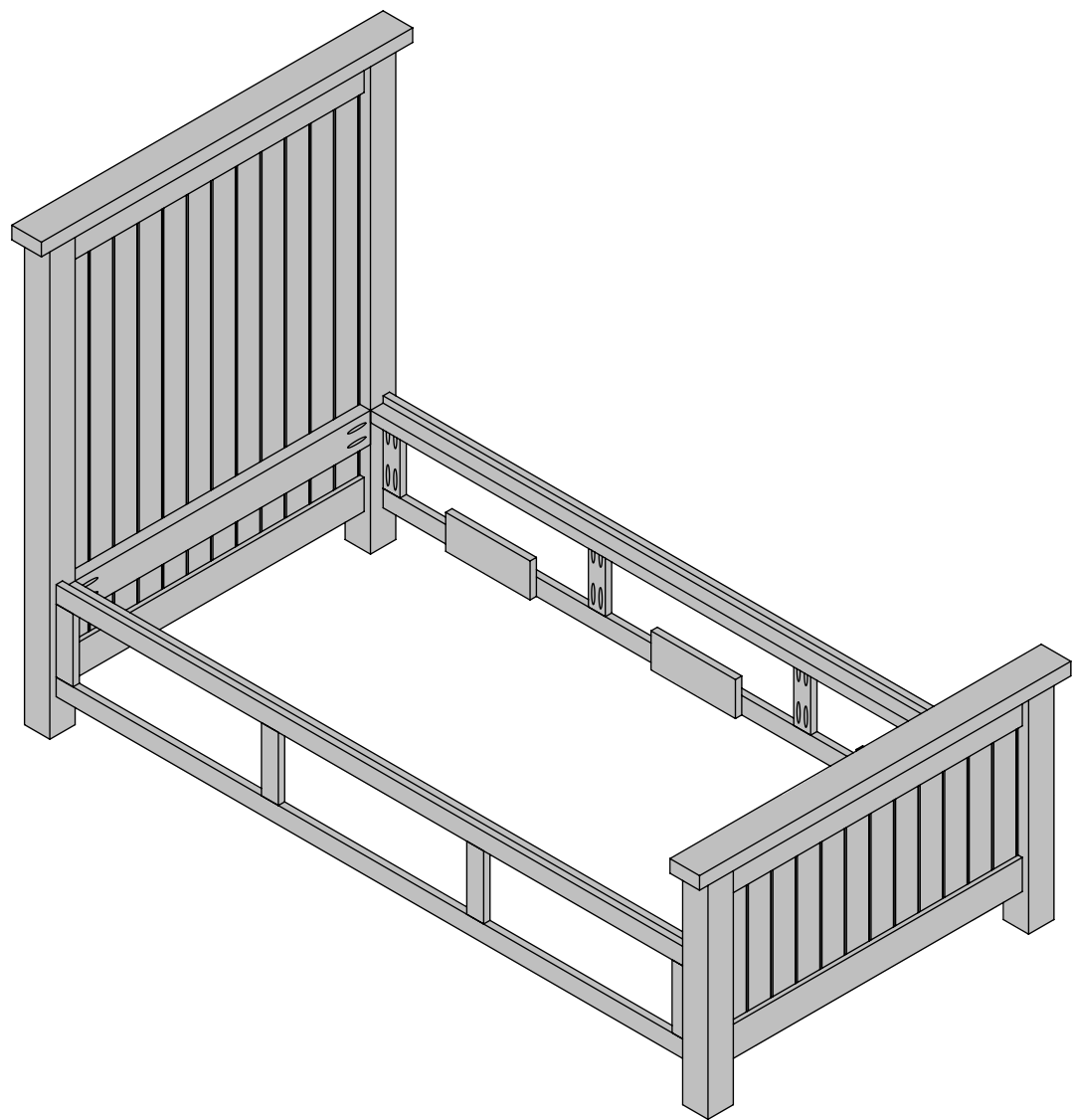
STEP 1: ATTACH BED RAILS WITH ROCKLER KEYHOLE BEDRAIL HARDWARE SO THAT SLAT SUPPORTS ARE FLUSH WITH CENTER SLAT RAIL.
