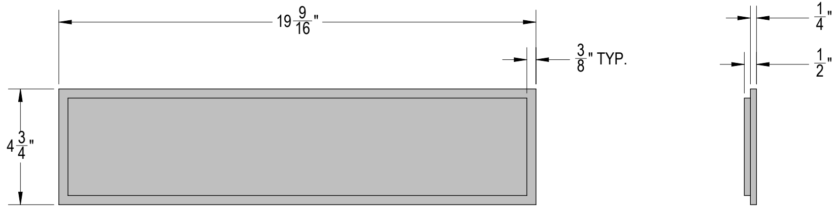
⑩ DRAWER FRONT PANEL MATERIAL: 1/2" MDF QTY: 6
