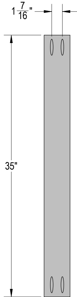
⑥ HEADBOARD / FOOTBOARD BOTTOM RAIL MATERIAL: POPLAR QTY: 2
