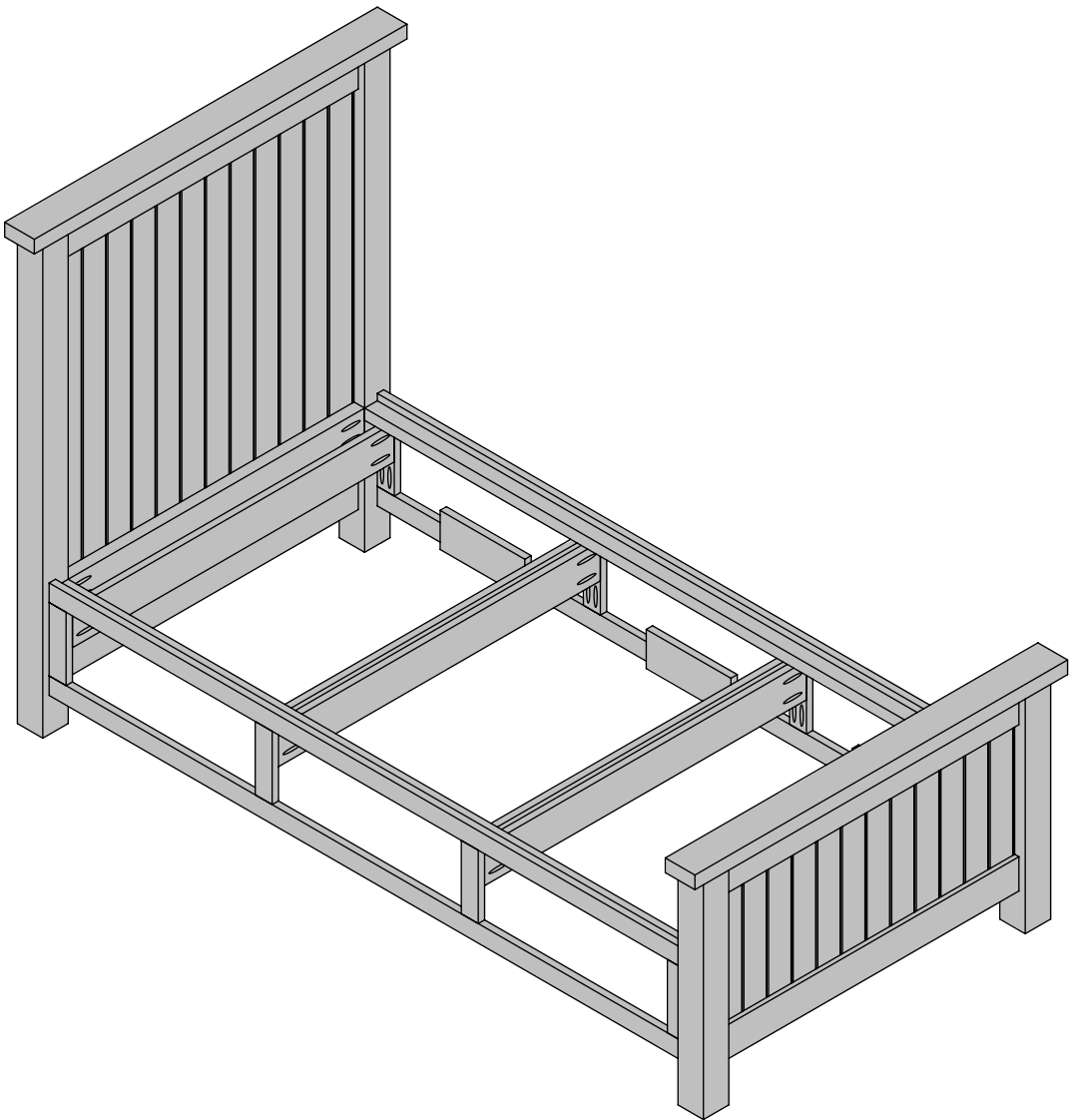
STEP 2: INSTALL DRAWER SLIDE SUPPORTS WITH 1-1/4" POCKETHOLE SCREWS. SUPPORTS SHOULD BE FLUSH WITH SIDES OF STILES AND BOTTOM OF SLAT SUPPORT.
