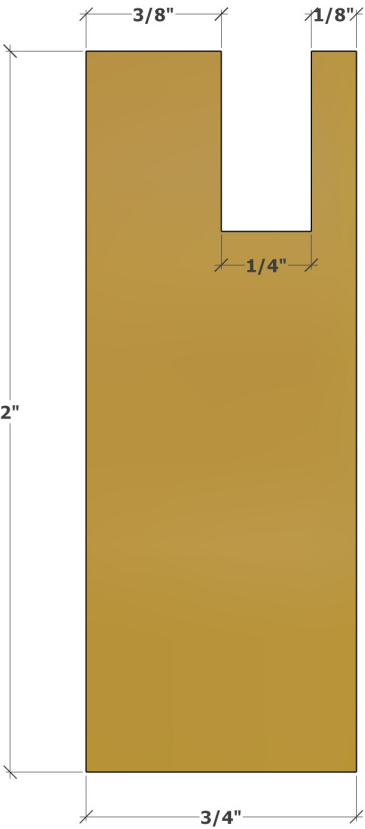
Door Rail - End View
