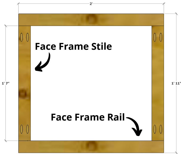
Face Frame - Back View
