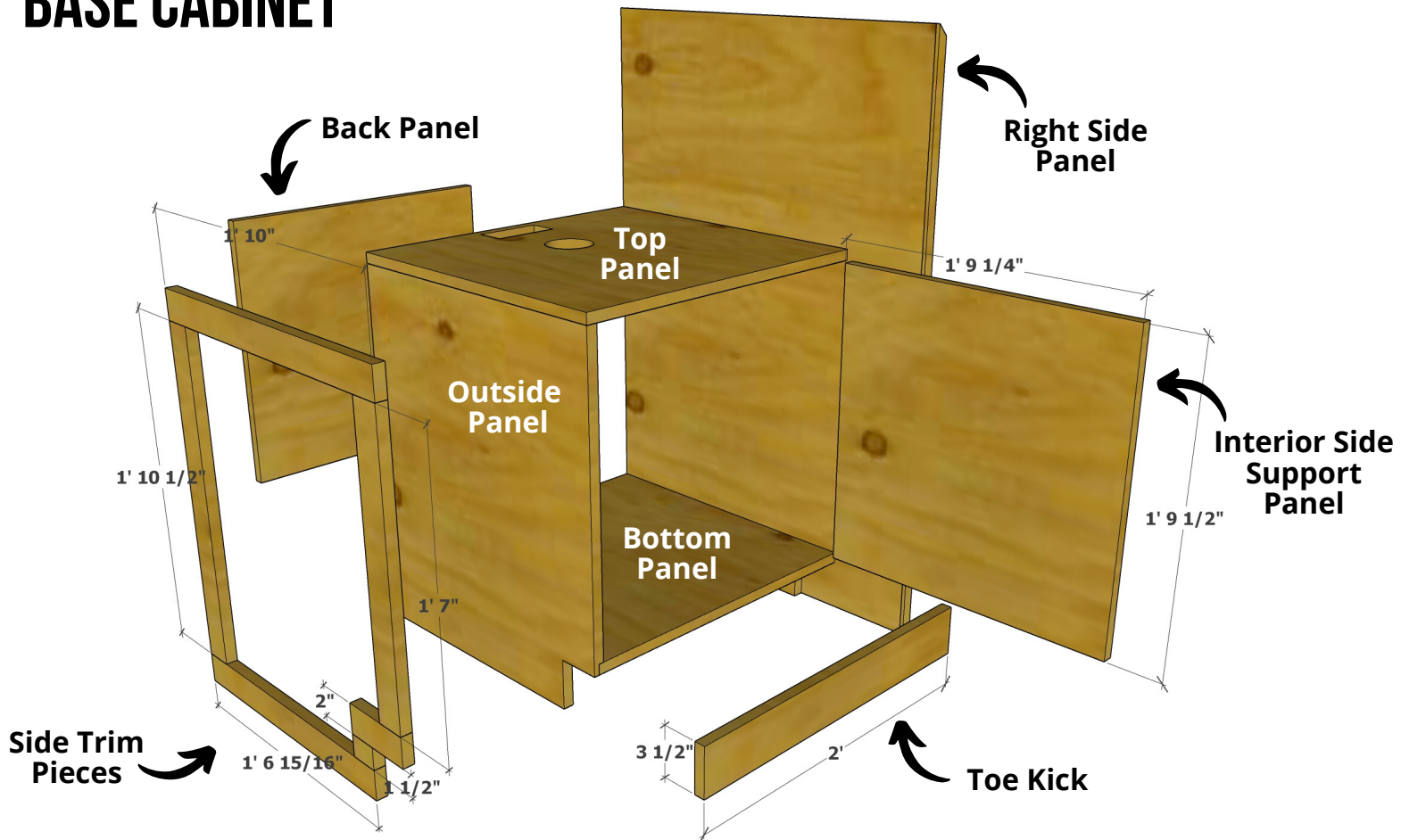
Base Cabinet - All Components Exploded
