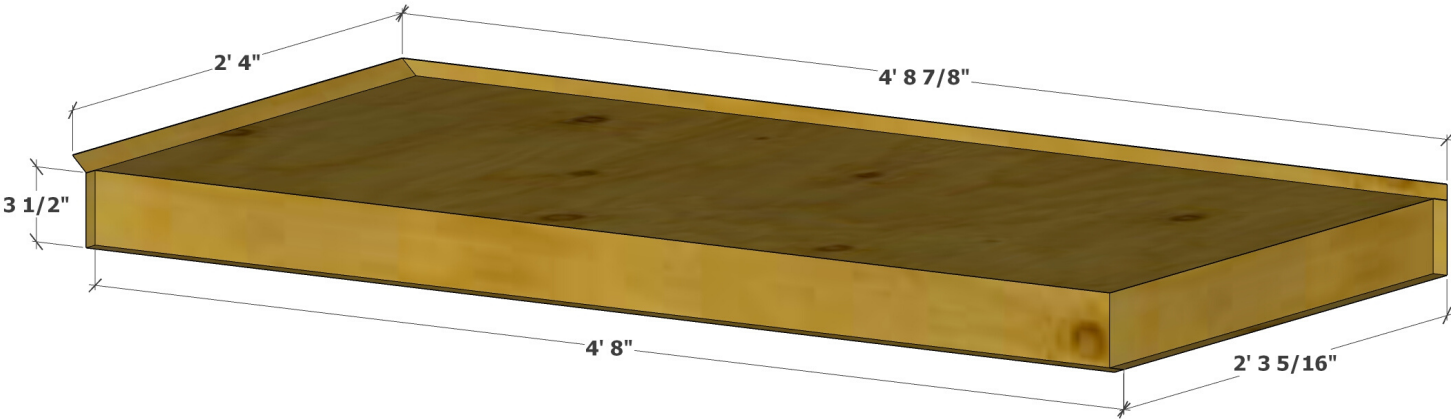
Folding Table - Front View
