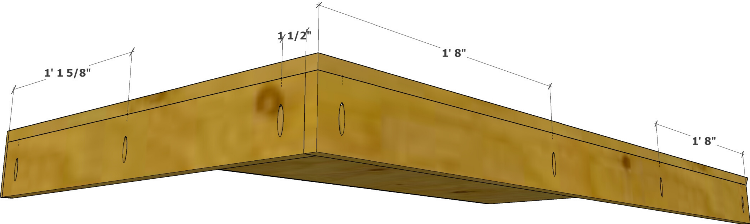
Folding Table - Back View
