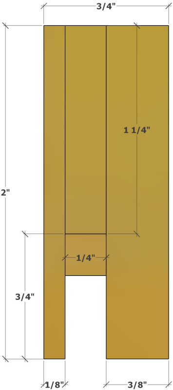
Door Stile - End View
