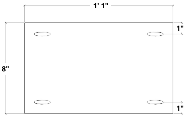
SIDE PANELS - QTY 2
